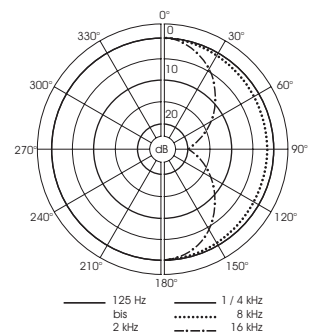
Polar patterns
